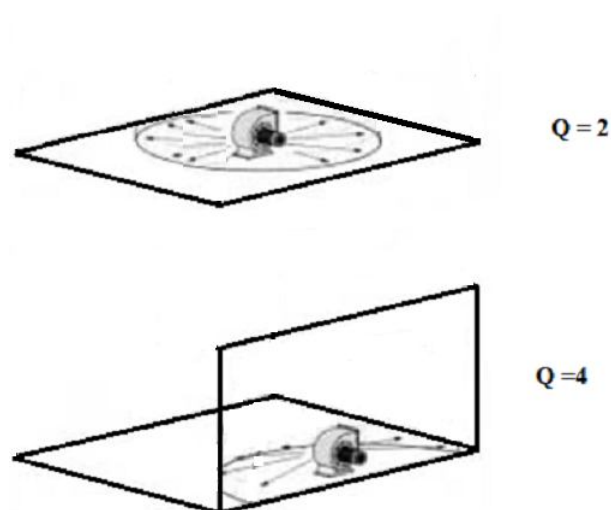
Fig 3: Schematic of two locations of fan in the acoustic lab along with the directivity factors( Q )
