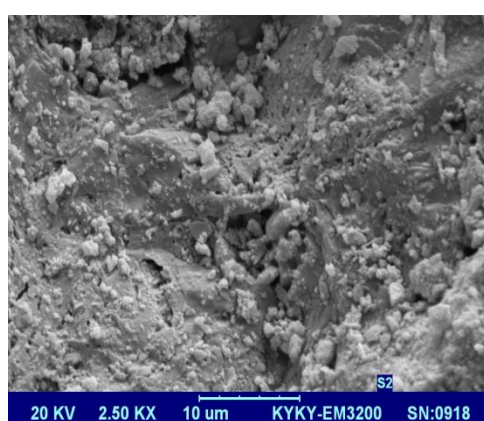
Fig.2: SEM image of steel slag
